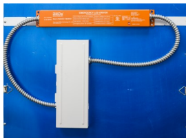
Emergency System Pre-installed (In 2X4 Installed but not attached to fixture)
